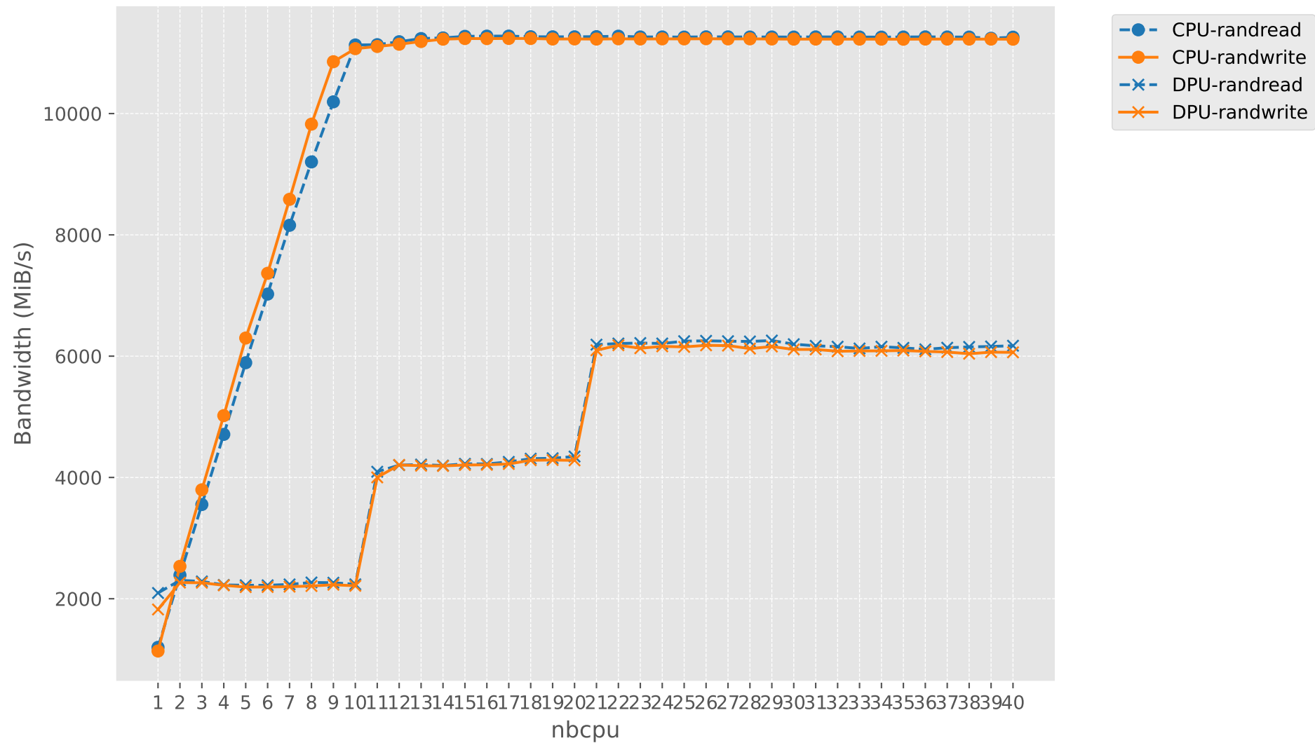
Bandwidth vs nbcpu (CPU vs DPU)
